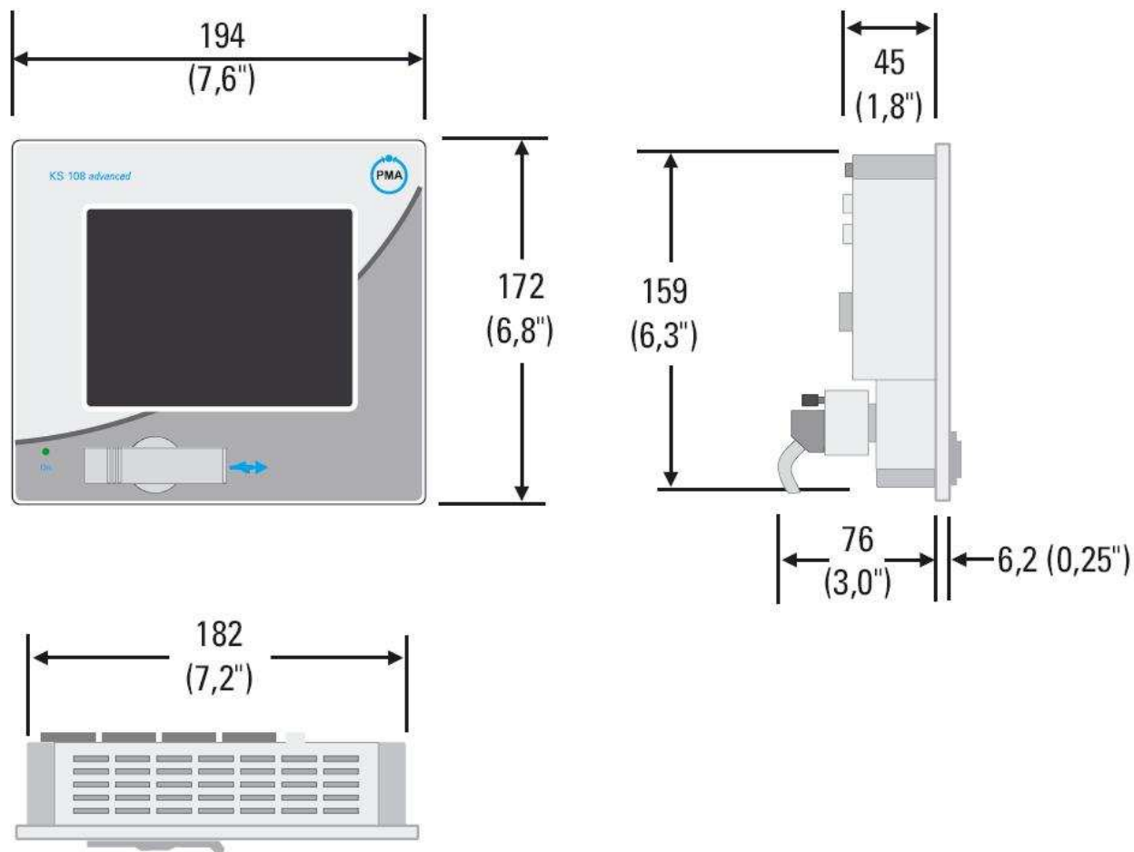
Fig. 1: Overall dimensions KS 108 easy
